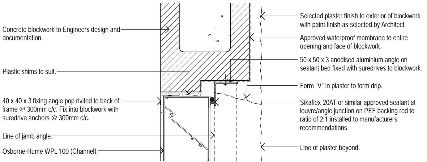
Model WPL 100 (Channel Frame) Typical Blockwall/Louvre Head Detail 01 Osborne-Hume Grilles & Louvres Ltd Scale 1:5
