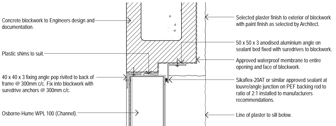
Model WPL 100 (Channel Frame) Typical Blockwall/Louvre Jamb Detail 02 Osborne-Hume Grilles & Louvres Ltd Scale 1:5
