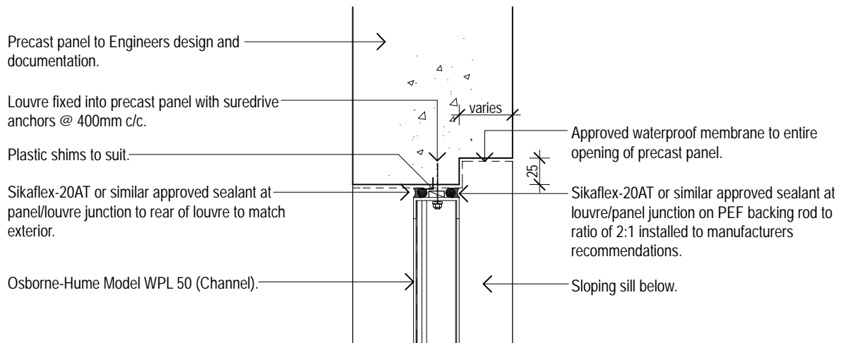
Model WPL 50 (Channel Frame) Typical Precast/Louvre Jamb Detail 02 Osborne-Hume Grilles & Louvres Ltd Scale 1:5
