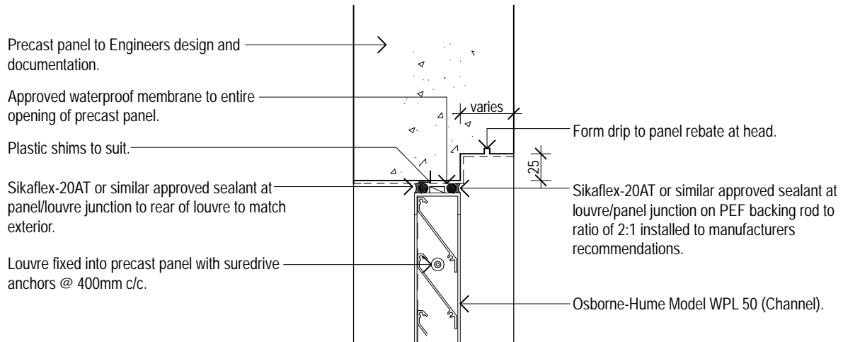
Model WPL 50 (Channel Frame) Typical Precast/Louvre Head Detail 01 Osborne-Hume Grilles & Louvres Ltd Scale 1:5
