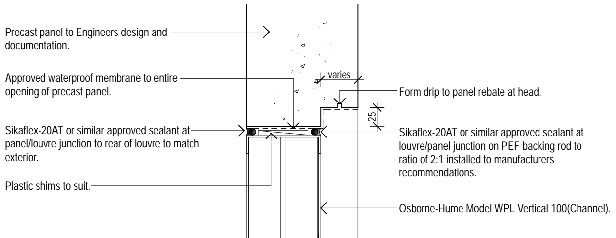
Model WPL Vertical 100 (Channel Frame) Typical Precast/Louvre Head Detail 01 Osborne-Hume Grilles & Louvres Ltd Scale 1:5
