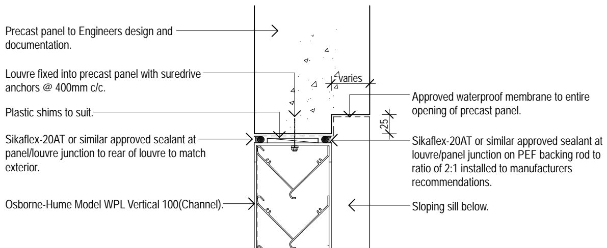
Model WPL Vertical 100 (Channel Frame) Typical Precast/Louvre Jamb Detail 02 Osborne-Hume Grilles & Louvres Ltd Scale 1:5
