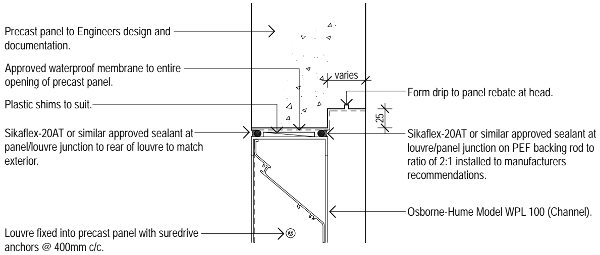
Model WPL 100 (Channel Frame) Typical Precast/Louvre Head Detail 01 Osborne-Hume Grilles & Louvres Ltd Scale 1:5
