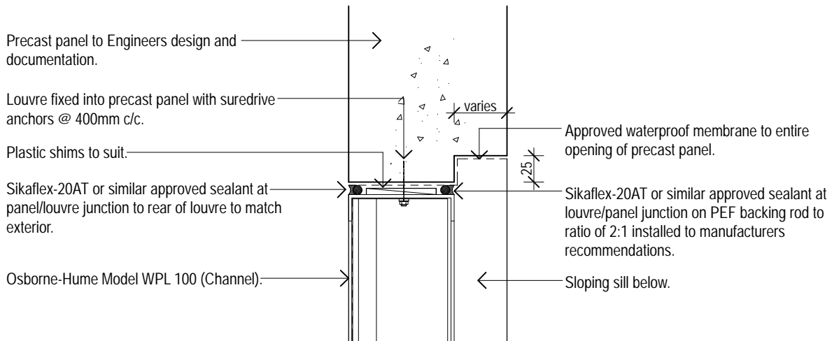
Model WPL 100 (Channel Frame) Typical Precast/Louvre Jamb Detail 02 Osborne-Hume Grilles & Louvres Ltd Scale 1:5
