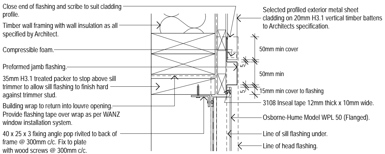
Model WPL 50 (Flanged Frame) Typical Horizontal Corrugate/Louvre Jamb Detail 02 Osborne-Hume Grilles & Louvres Ltd Scale 1:5
