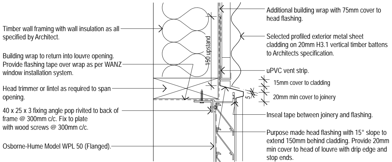
Model WPL 50 (Flanged Frame) Typical Horizontal Corrugate/Louvre Head Detail 01 Osborne-Hume Grilles & Louvres Ltd Scale 1:5
