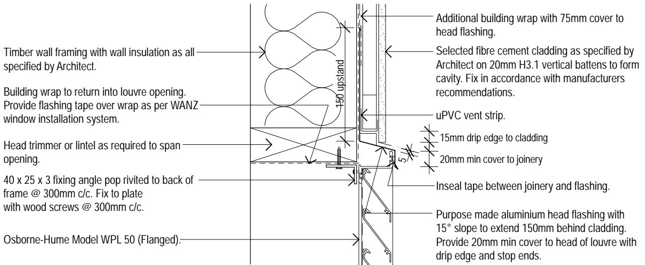
Model WPL 50 (Flanged Frame) Typical Fibre Cement/Louvre Head Detail 01 Osborne-Hume Grilles & Louvres Ltd Scale 1:5
