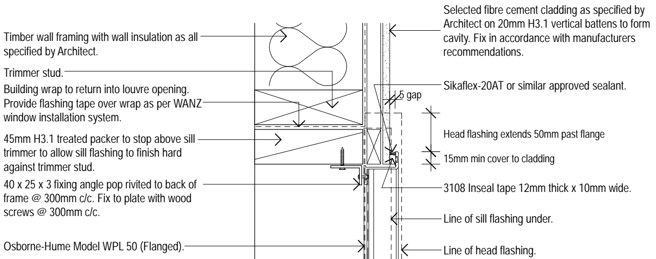
Model WPL 50 (Flanged Frame) Typical Fibre Cement/Louvre Jamb Detail 02 Osborne-Hume Grilles & Louvres Ltd Scale 1:5
