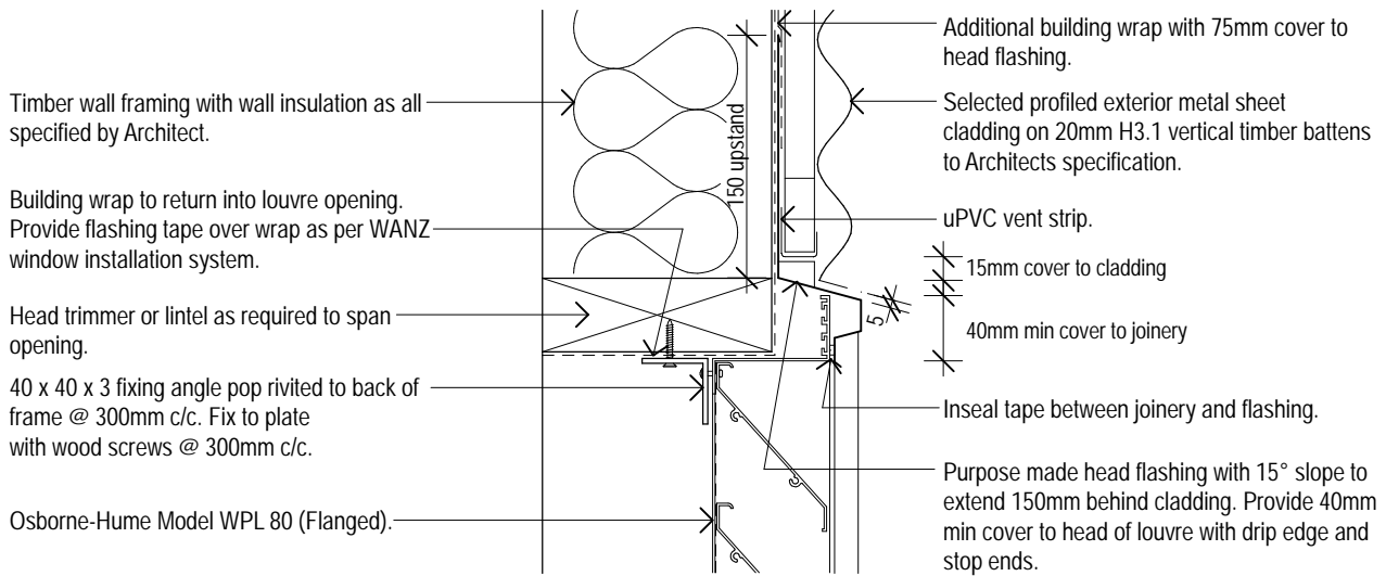
Model WPL 80 (Flanged Frame) Typical Horizontal Corrugate/Louvre Head Detail 01 Osborne-Hume Grilles & Louvres Ltd Scale 1:5
