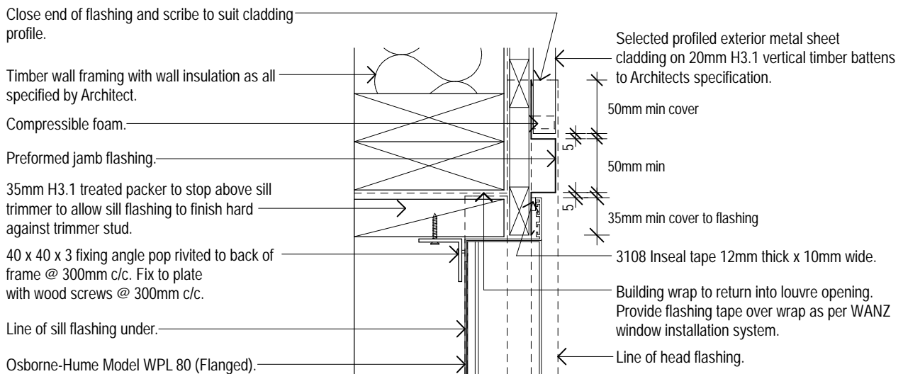
Model WPL 80 (Flanged Frame) Typical Horizontal Corrugate/Louvre Jamb Detail 02 Osborne-Hume Grilles & Louvres Ltd Scale 1:5
